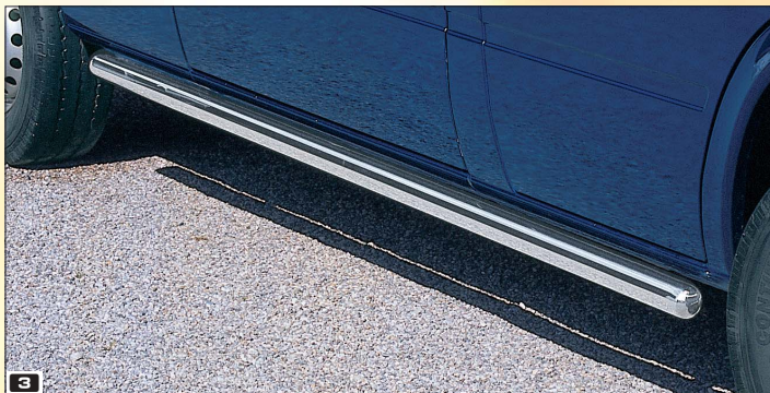
3 Side bar Flankenschutzrohr Stainless steel / Edelstahl Wheel base / Radstand 3000 mm 150 4050 Wheel base / Radstand 3550 mm 150 4051 Wheel base / Radstand 4025 mm 150 4052
